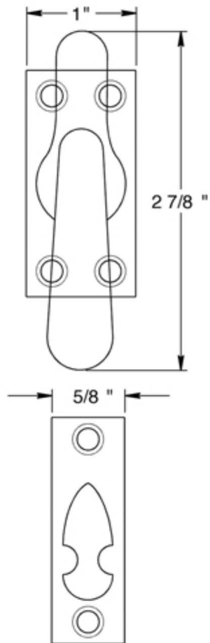
FRONT VIEW
