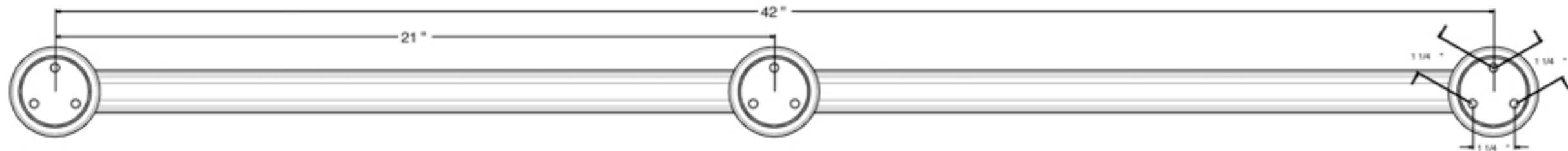
BOTTOM VIEW
