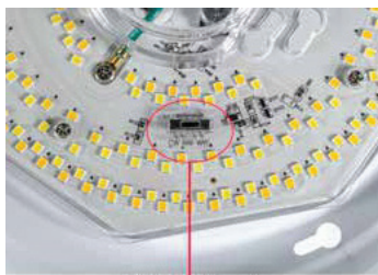
Switch to change Color Temperature from 3000K, 4000K or 5000K
