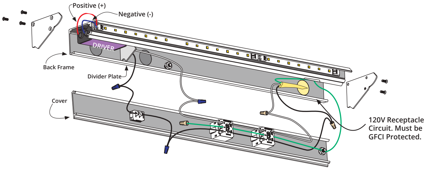
18-1/2" Fixture Shown
