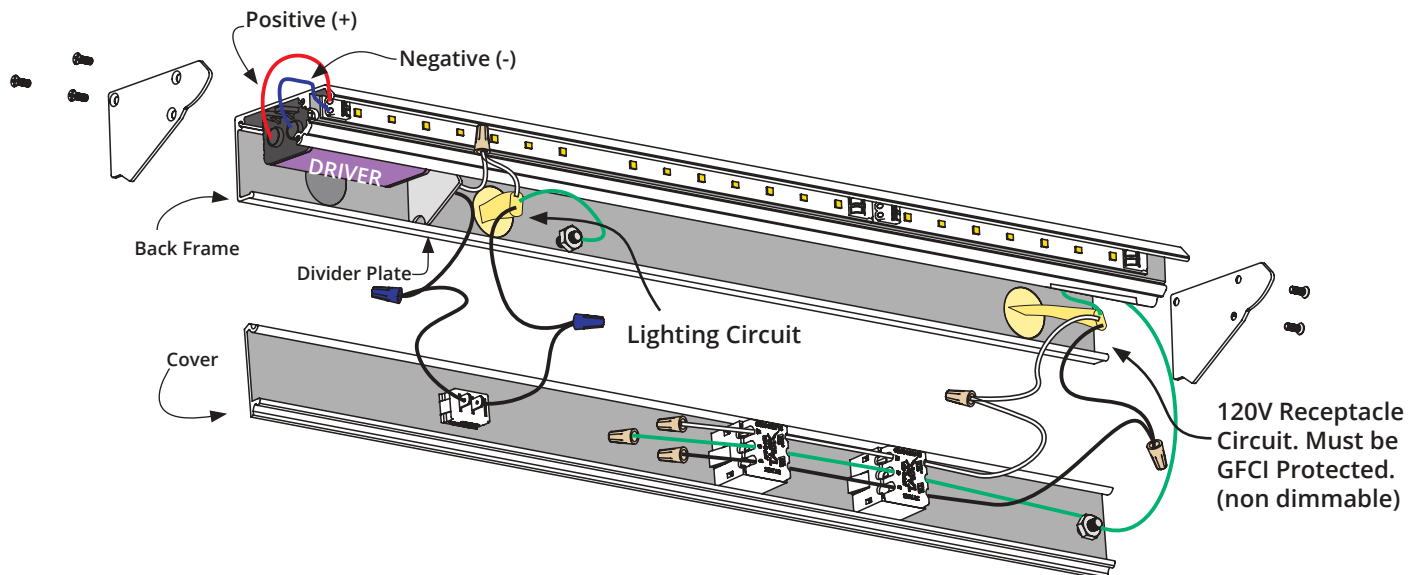
18-1/2" Fixture Shown
